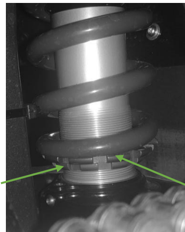
Spline nut
